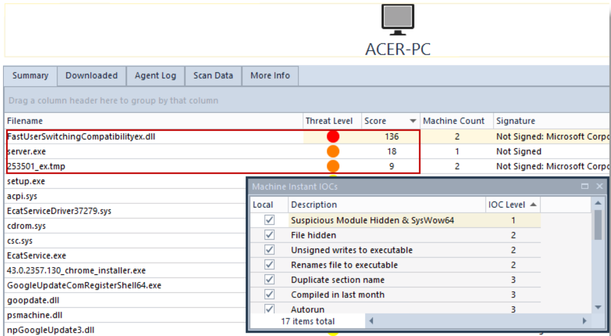
Figure 4 – Suspicious Modules Running on ACER-PC
