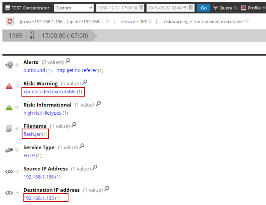
Figure 9 – Evidence of Suspicious File Downloaded after Link Clicked
