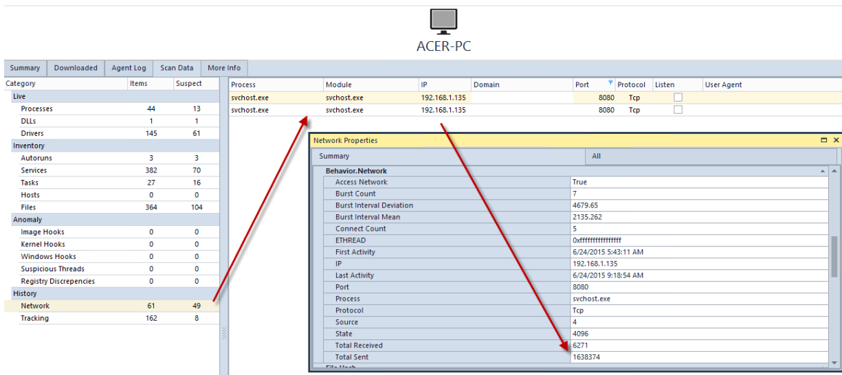
Figure 6– Identify Process Responsible for Gh0st C2 Traffic
