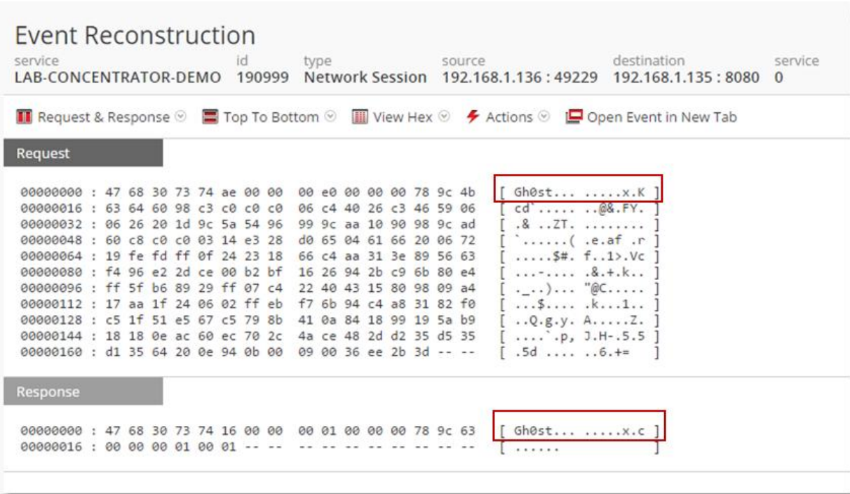
Figure 2 – Reconstruction of Gh0st Payload in RSA Security Analytics
