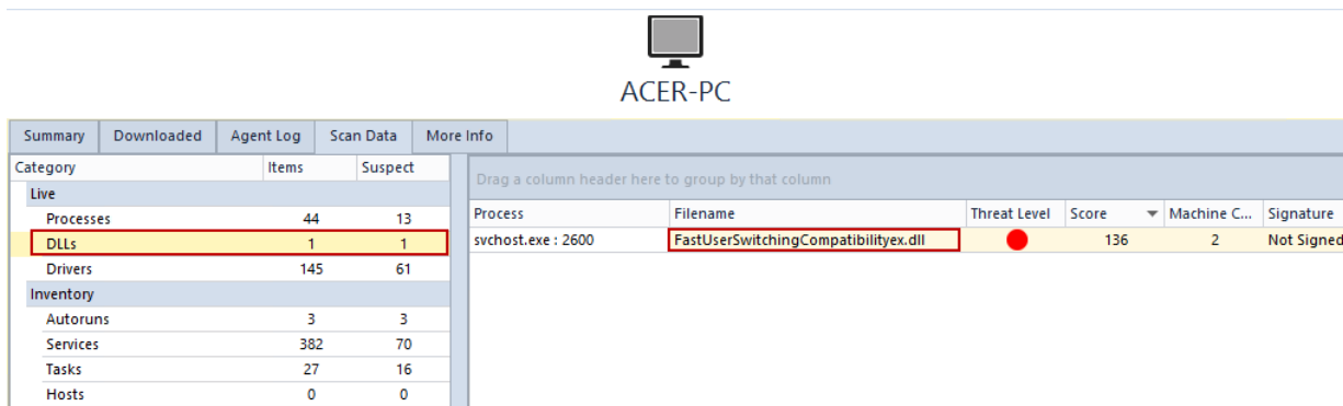
Figure 7 – Scan Data Showing svchost.exe Loading a Suspicious Module
