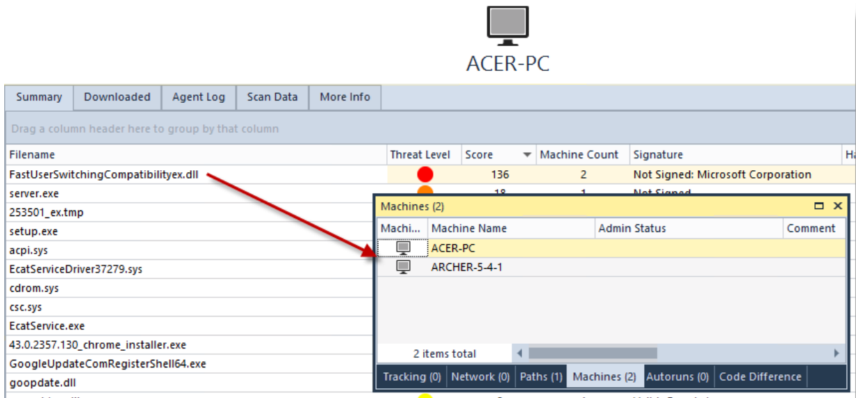
Figure 5 – Take Note of Other Computers with the Same Module
